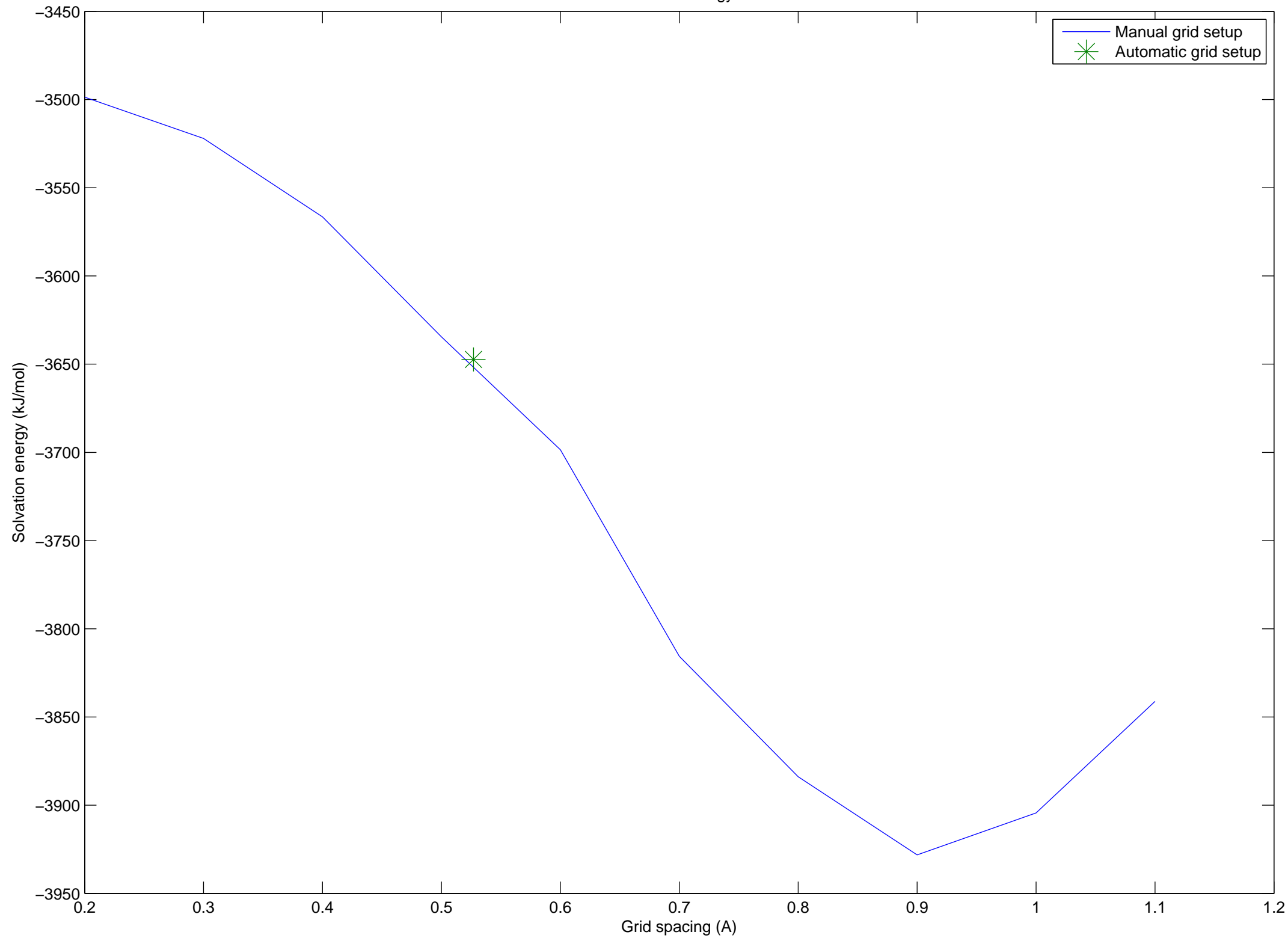
1BBL solvation energy results
